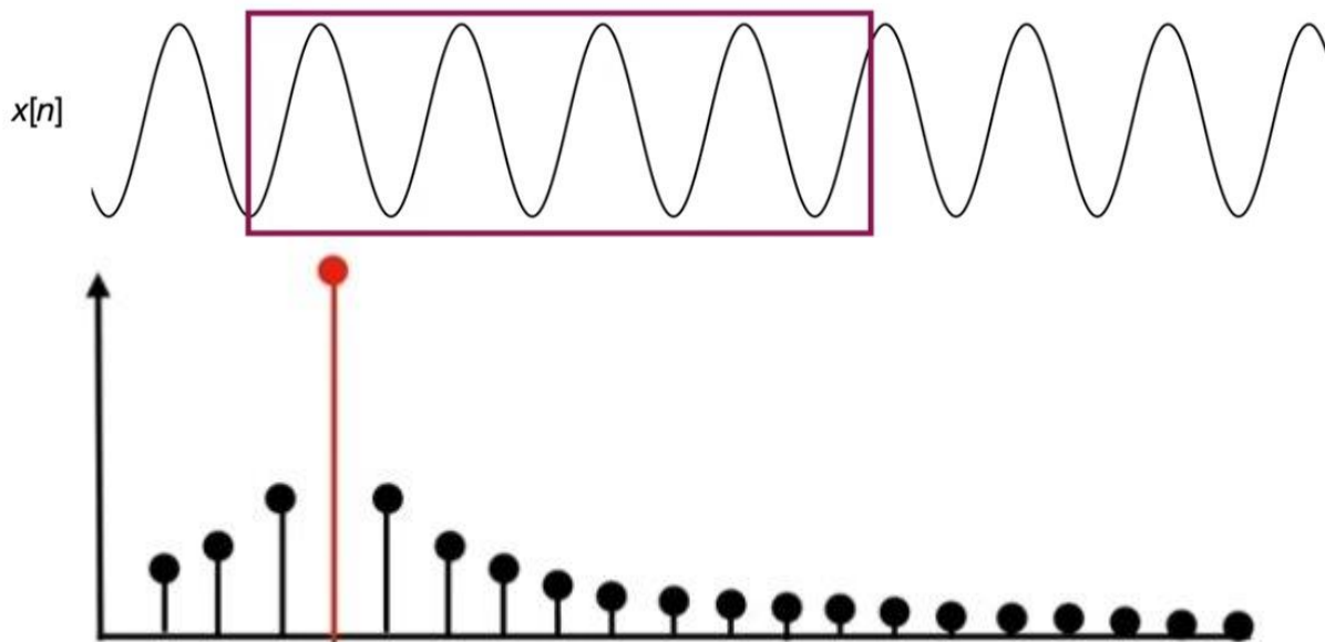
Figure 5: Window of a sinusoid with a non-integer number of periods (top) with its resulting FFT spectrum (bottom).
