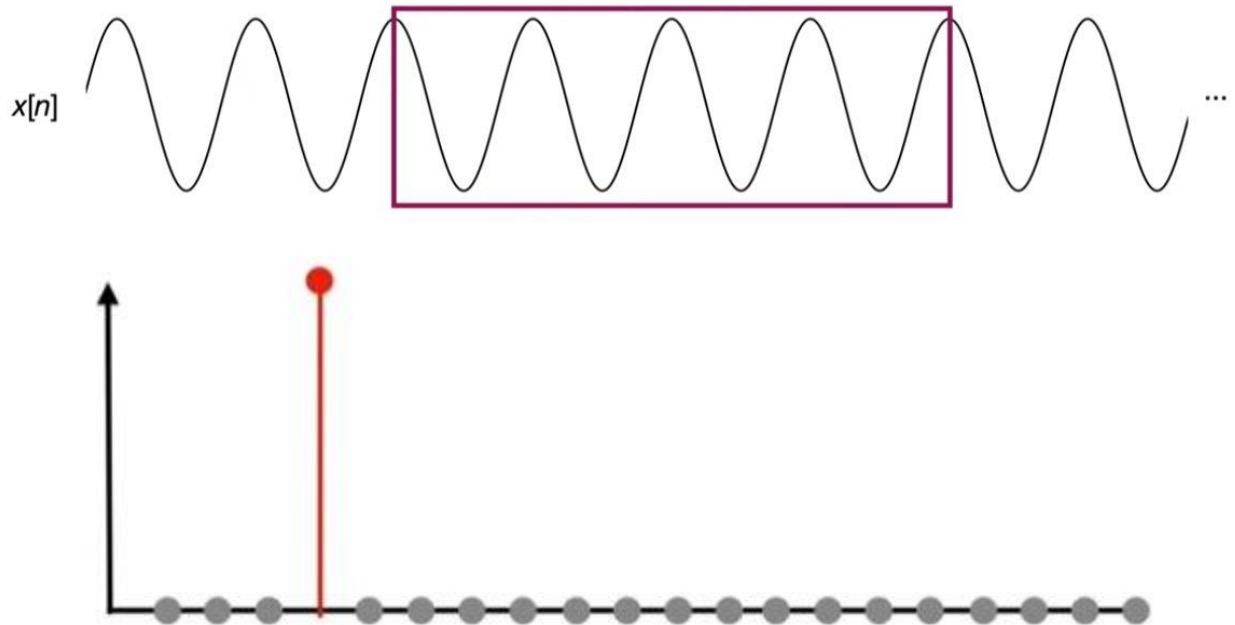
Figure 4: Window of a sinusoid with an integer number of periods (top) with its resulting FFT spectrum (bottom).
